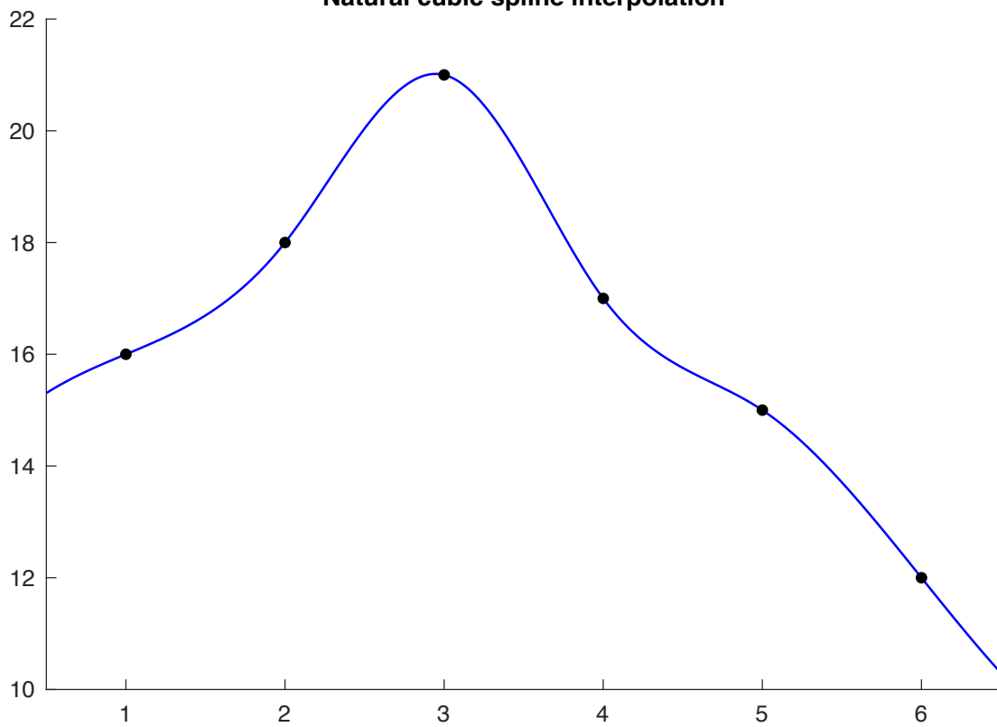
Natural cubic spline interpolation
