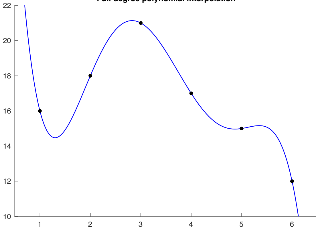
Full degree polynomial interpolation
