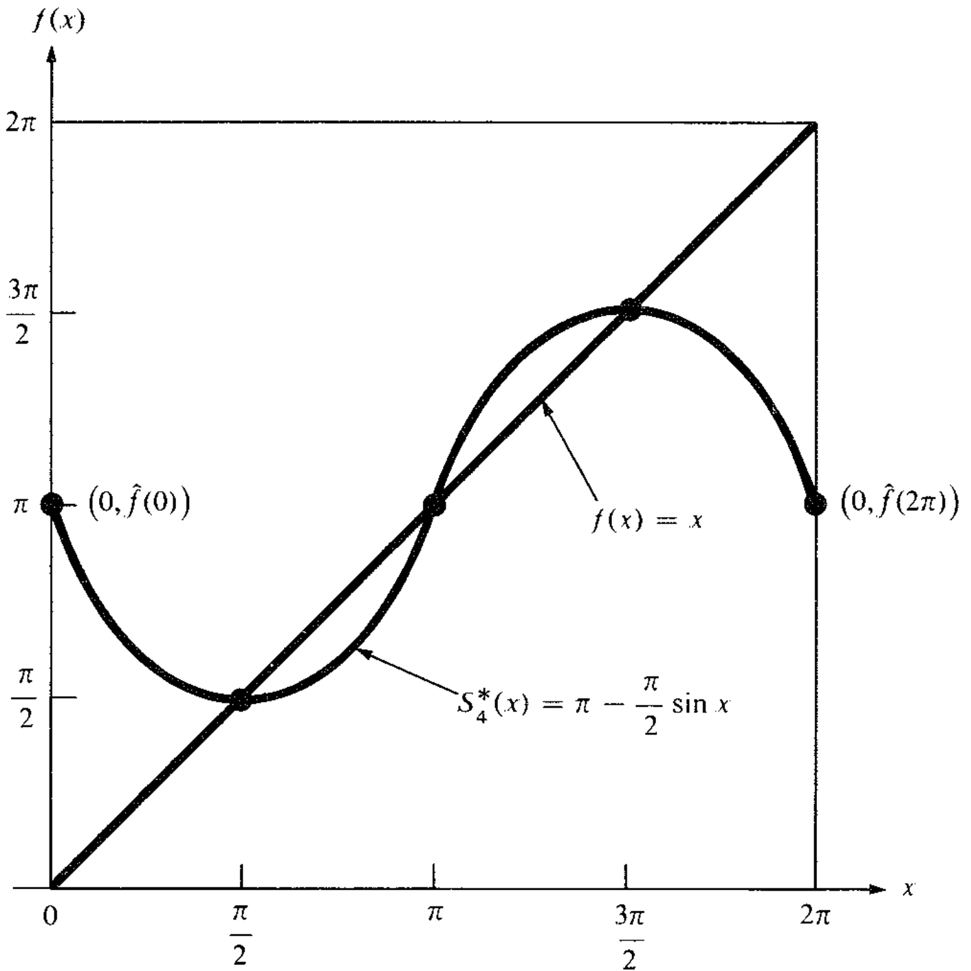
Trigonometric Interpolation for f(x) = x , 0 \leq x \leq 2\pi .
