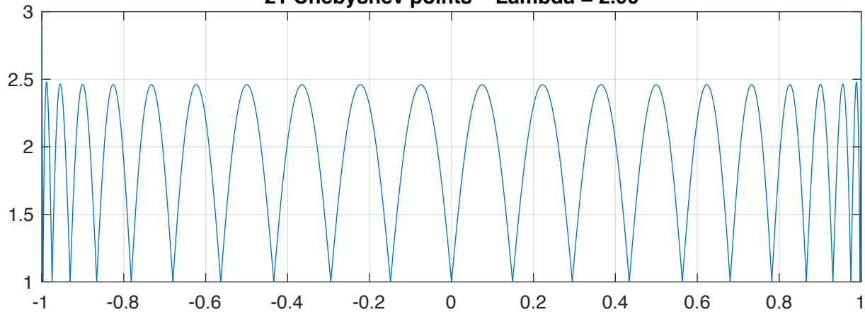
21 Chebyshev points Lambda = 2.90
