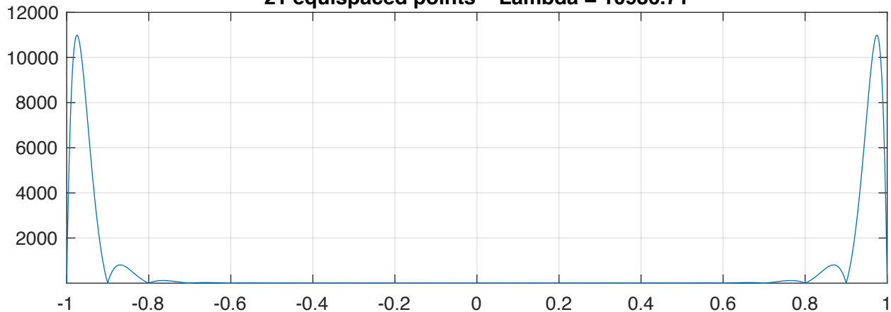
21 equispaced points Lambda = 10986.71
