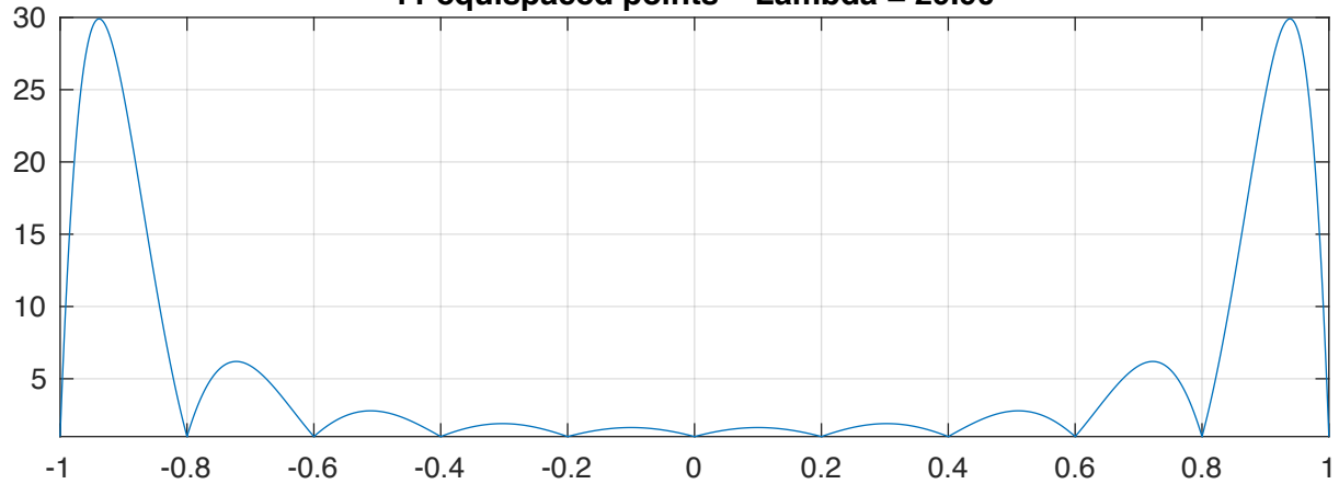
11 equispaced points Lambda = 29.90
